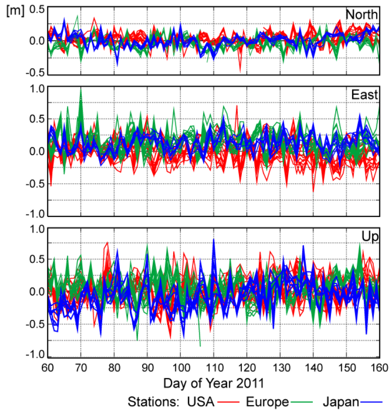
Fig. 2: Differences with respect to reference solutions for PPP results using orbits and clock corrections from the GPS broadcast messages for stations in USA, Europe and Japan. Each trace represents a different station.
