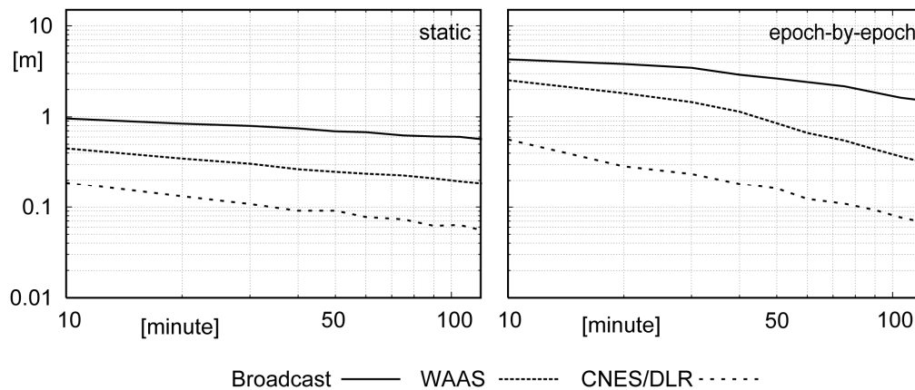
Fig. 6: RMS values of 3D-coordinates for observation times of 10 to 120 minutes for static observation data processed in static or simulated kinematic mode
