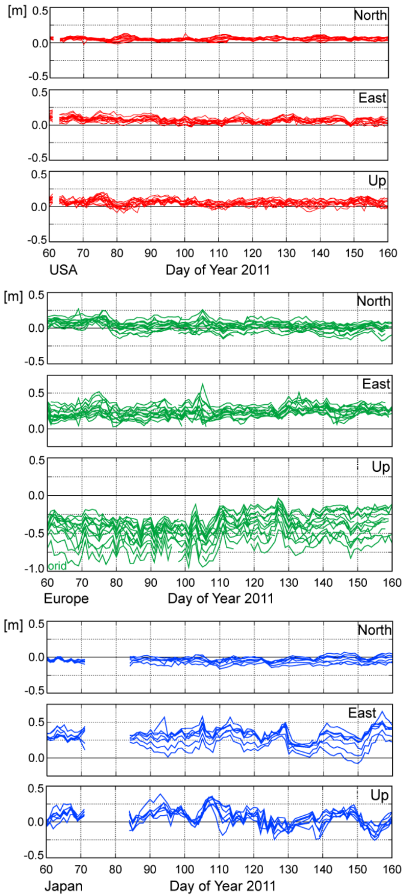
Fig. 3: Difference with respect to reference solutions for PPP results using SBAS products: WAAS in the USA, EGNOS in Europe, and MSAS in Japan. Each trace represents a different station
