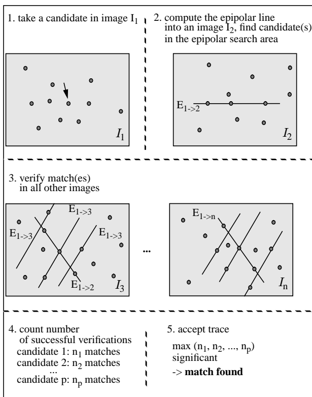
Figure 1: Computation scheme for the automatic establishment of correspondences via epipolar line intersection
