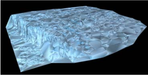
Figure 10: Terrestrial laserscanner glacier front surface model of Jakobshavn Isbræ, July 2007
