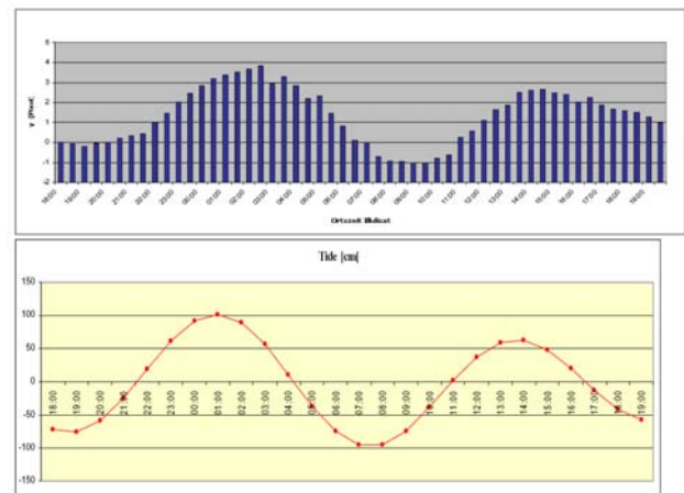
Figure 6: Trajectory from image sequence tracking (top), tidal curve (bottom)
