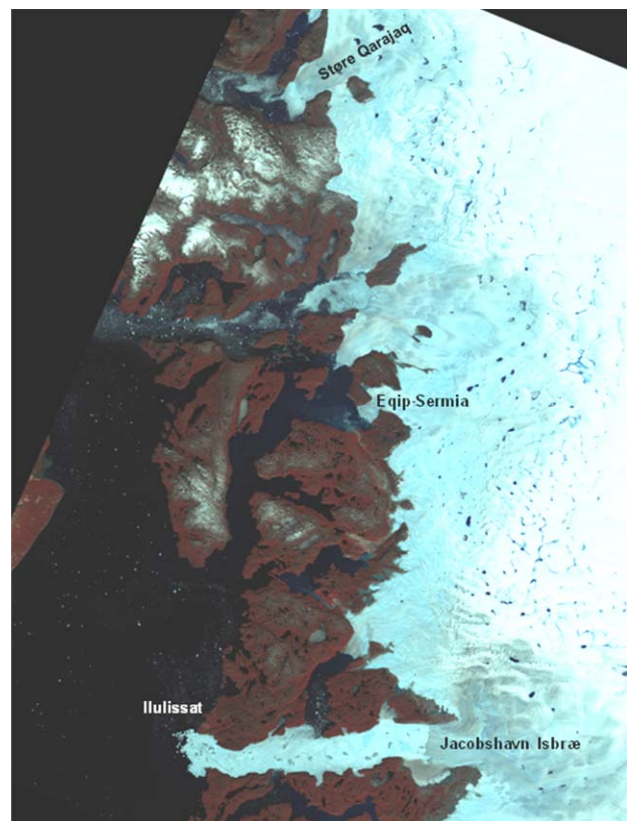
Figure 1: West Greenland with Støre Qarajaq, Eqip Sermia and Jacobshavn Isbræ glaciers (Landsat 2001 false color image)
