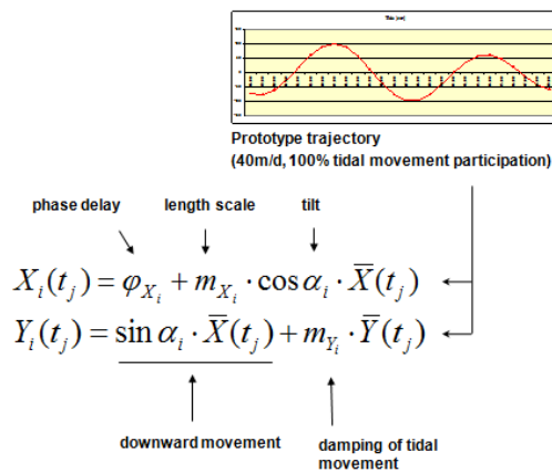
Figure 7: Trajectory matching approach
