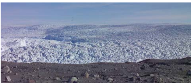
Figure 4: Image of Jacobshavn Isbræ glacier front area (Maas et al., 2004), observation point marked in Figure 3
