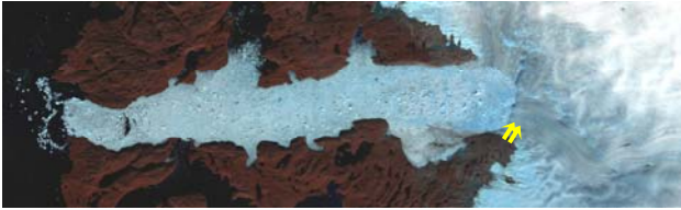
Figure 3: Jacobshavn Isbræ and Kangia Fjord, 2004+2007 observation points (arrows)
