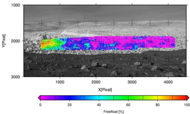
Figure 8: Tidal movement of the glacier in percent of free float
