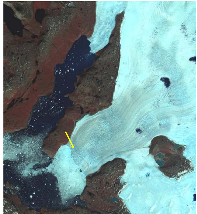
Figure 11: Støre Qarajaq (2001 Landsat false color image), 2007 observation point
