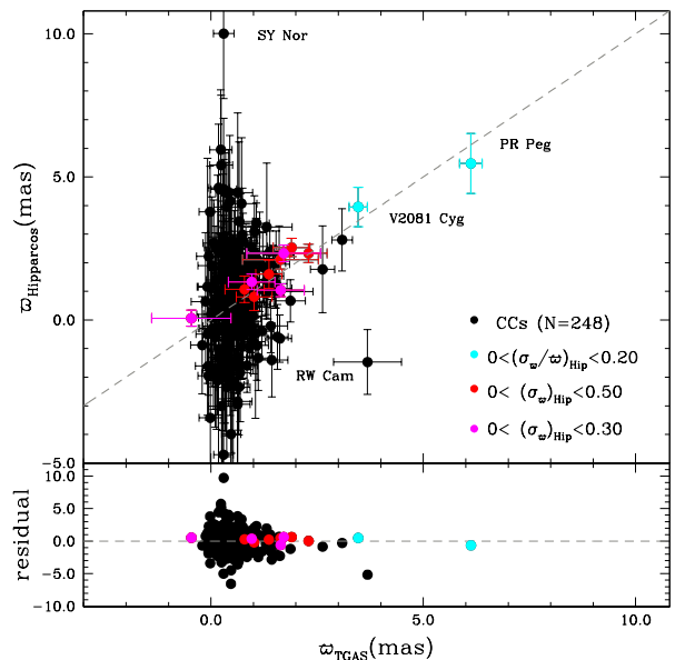
Fig. 5. Comparison between Hipparcos and TGAS parallaxes, obtained from a sample of 248 classical Cepheids which have both measurements. Red and magenta filled circles represent stars with (\sigma_{\varpi}/\varpi)_{\text{Hipparcos}} < 0.50 and 0.30 mas, respectively, cyan filled circles are two stars with (\sigma_{\varpi}/\varpi)_{\text{Hipparcos}} < 0.20 , namely, V2081 Cyg and PR Peg. A dashed line shows the bisector. Residuals are: TGAS – Hipparcos parallax values.
