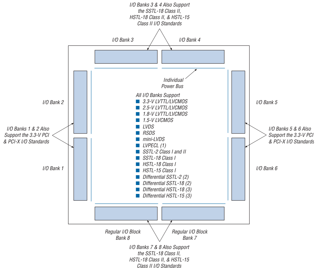
Figure 11–2. I/O Banks in EP2C15, EP2C20, EP2C35, EP2C50 &amp; EP2C70 Devices
