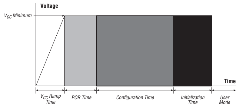
Figure 4–3. Cyclone II Wake-Up Time
