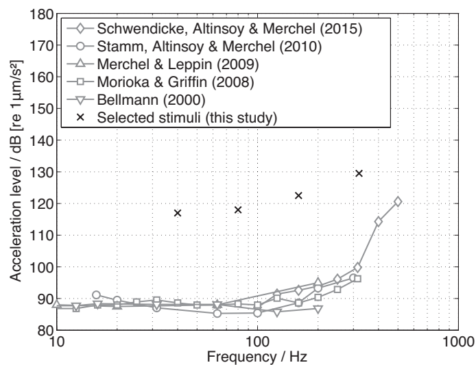
Figure 3 – Selected reference stimuli and perception threshold for vertical seat vibrations [2-6].
