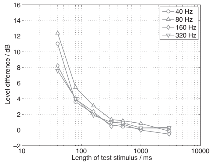
Figure 6 – Difference between the adjusted level of the test vibration and the level of the reference vibration (mean) as a function of test stimulus duration for all four frequencies.
