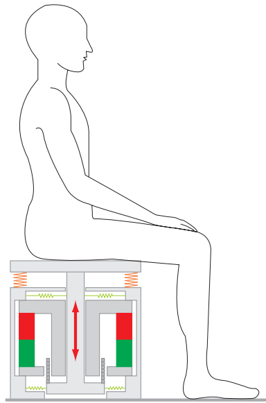
Figure 1 – Vibration chair with electrodynamic exciter.
