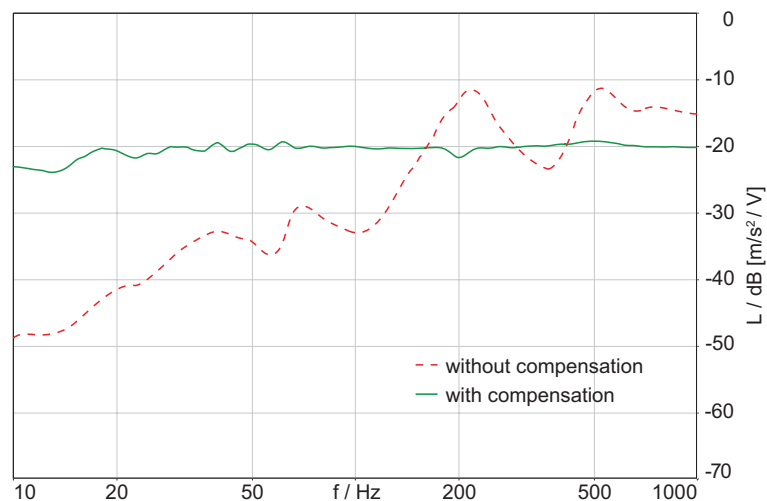
Figure 2 – Body-related transfer functions (FFT 65536, 1/24th octave intensity averaging) measured at the seat surface of the vibration chair, with and without compensation.
