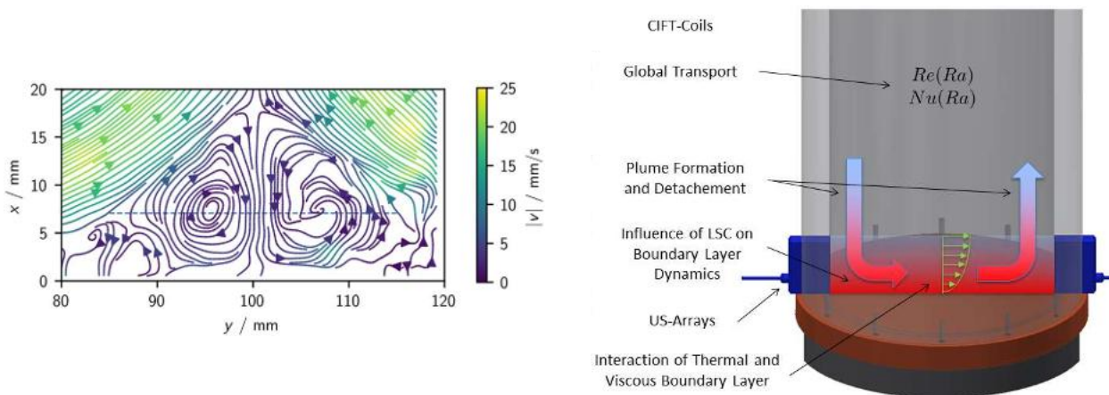
Super-resolution vector flow imaging of a recirculation area in a liquid metal convection.
