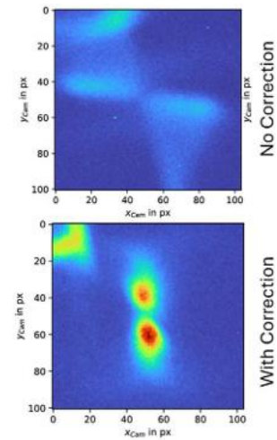
Fig. 3: Top: Particle image with aberrations due to refraction at drop surface Bottom: Particle image with Adaptive-Optical Correction
