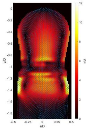
Fig. 2: Measured flow field in Taylor bubble
