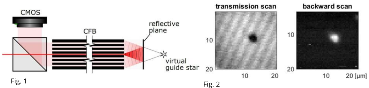
Left: Scheme virtual guide star calibration. Right: Endoscopic scan of fluorescent particle with diameter of 1 \mu\text{m} .
