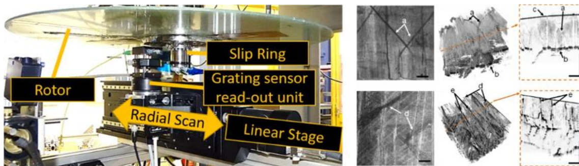
Diffraction Grating Sensors measuring in- and out-of-plane FRP rotor deformation field and vibration at >270 m/s with 20 \mu\epsilon and 15 \mu\text{rad} precision (left). OCT images of internal FRP rotor structure, showing delamination (b) and cracks (e) (right) due to overload.
