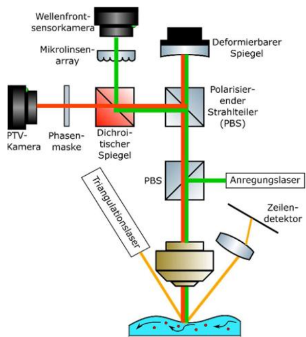
Fig. 2: Schematic diagram of the overall system with HS wavefront sensor, water level measurement using triangulation, deformable mirror, and 3D PTV system
