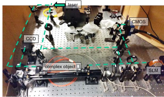
Digital Optical Phase Conjugation
