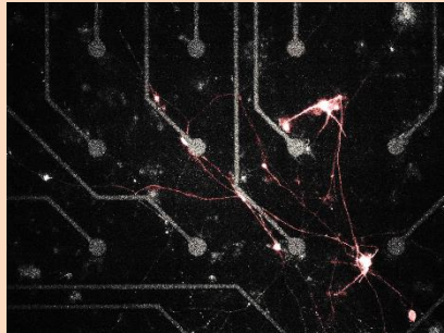
Neural Network
