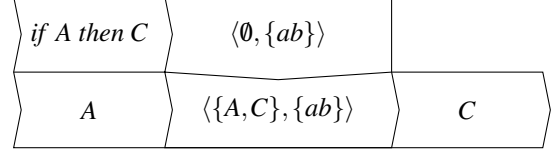
Figure 3: Modus ponens inference in WCS.
