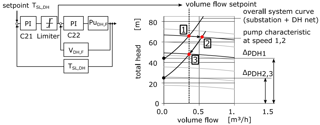
Figure 2: Left: Cascade controller for the feed-in temperature T_{SL,DH} , Right: Characteristic curves of the feed-in pump Pu_{DH,F} and the operation points 1..3 during the control action of C22 reacting on a step of \Delta p_{DH} (1 – Starting point, 2 – after step of \Delta p_{DH} without reaction of C22, 3 – final stage after correction of the pump speed)
