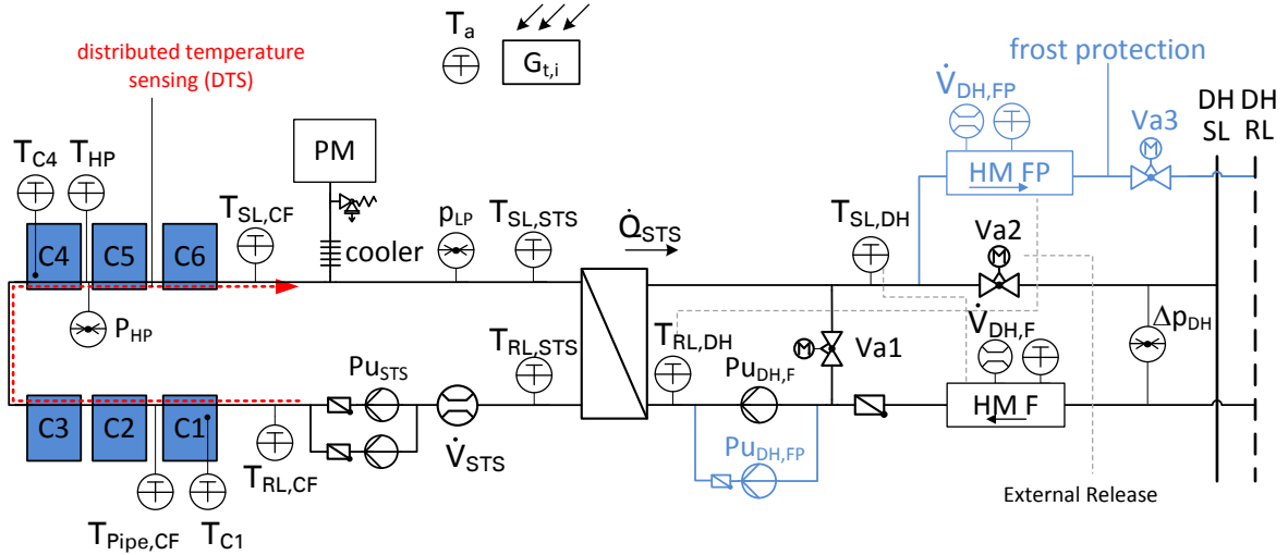
Figure 1: Schematic of the feed-in substation ( T_a – ambient temperature, C – collector, CF – collector field, DH – district heating, HM – heat meter, F – feed-in, FP – frost protection, HP – highest point, LP – lowest point, PM – pressure maintenance, Pu – pump, Va – valve, STS – solar thermal system)
