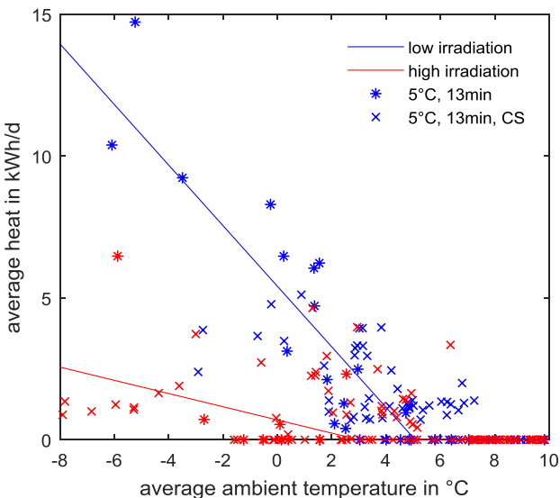
Figure 6: Statistical evaluation of the frost protection season in winter 2016/17 and 2017/18, daily average, low irradiation < 1,2 \text{ kWh}/(\text{m}^2 \text{ d}) in collector plane \leq high irradiation
