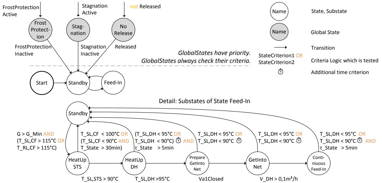
Figure 3: State diagram of the net feed-in substation with detailed sub-states of the state Feed-in Released – External release signal is true and feed-in allowed G_Min – minimal radiation threshold calculated on basis of the collector curve The criteria for Stagnation and Frost protection are discussed in the corresponding section.
