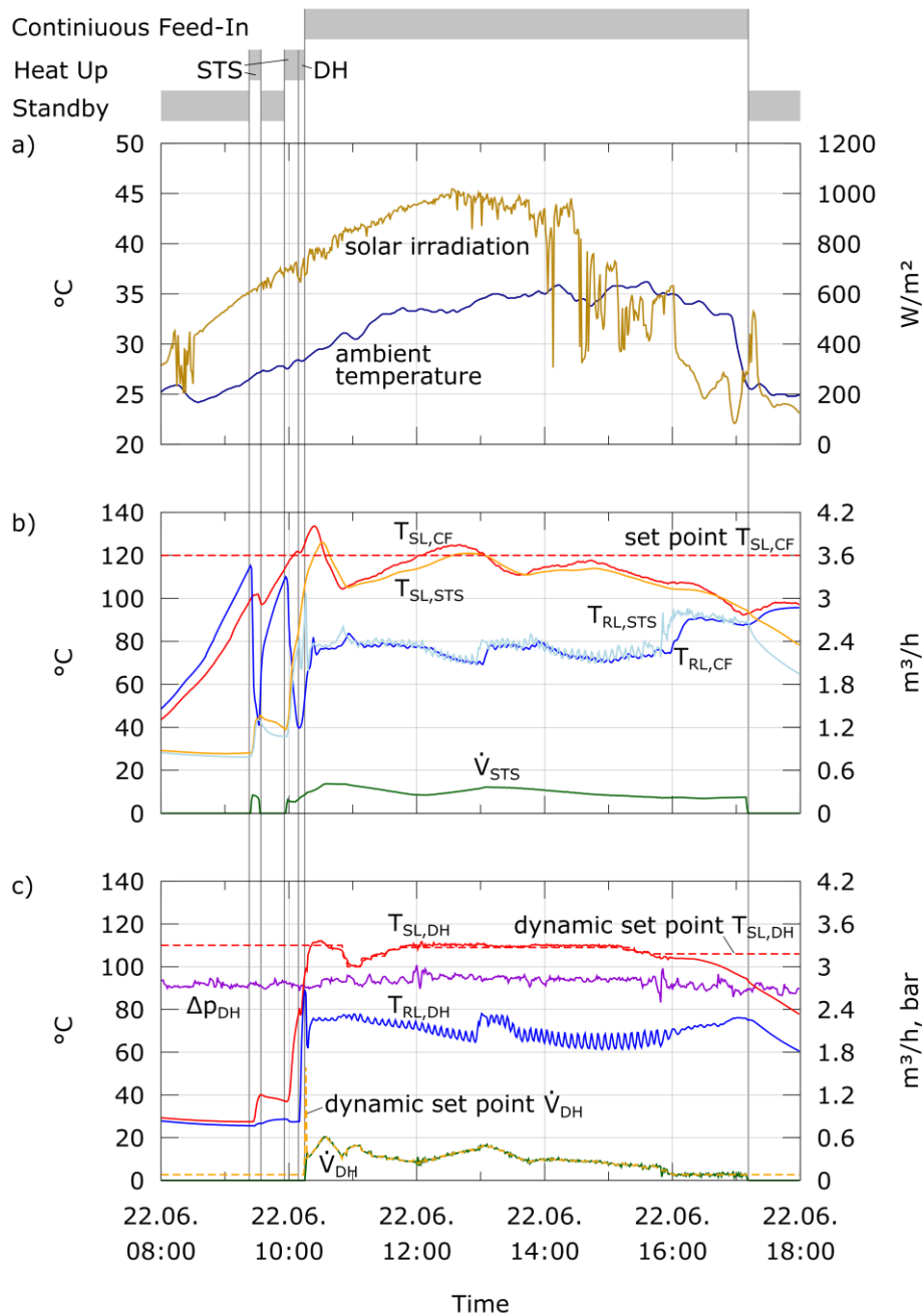
Figure 4: Measurement data for state Feed-in, a) ambient, b) solar system, c) district heating side
