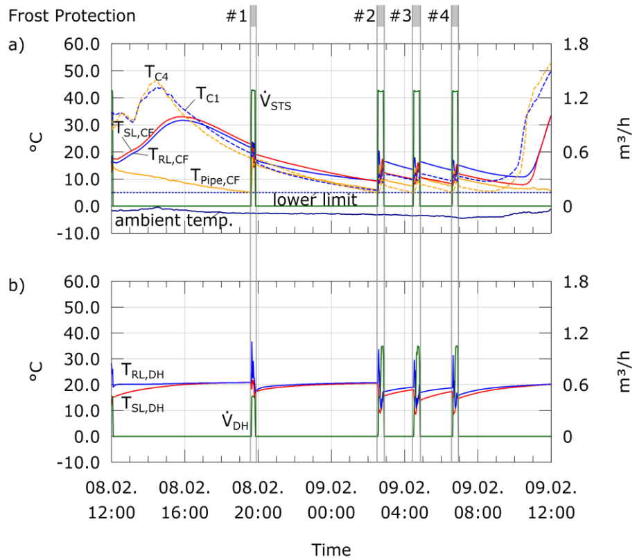
Figure 5: Measurement data for state Frost Protection, a) solar system, b) district heating side
