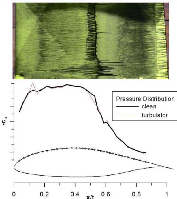
Fig. 4: Flow visualization and pressure distribution in wind tunnel
