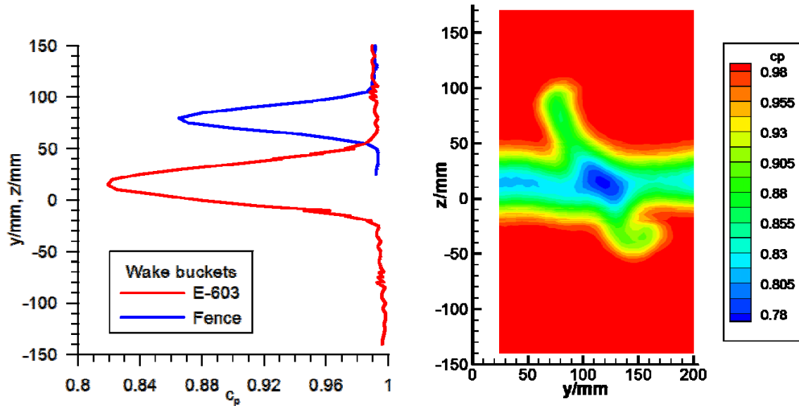
Fig. 9: Wake of a fence, vortex sheet downstream of the slightly tapered wing distorts the wake flow
