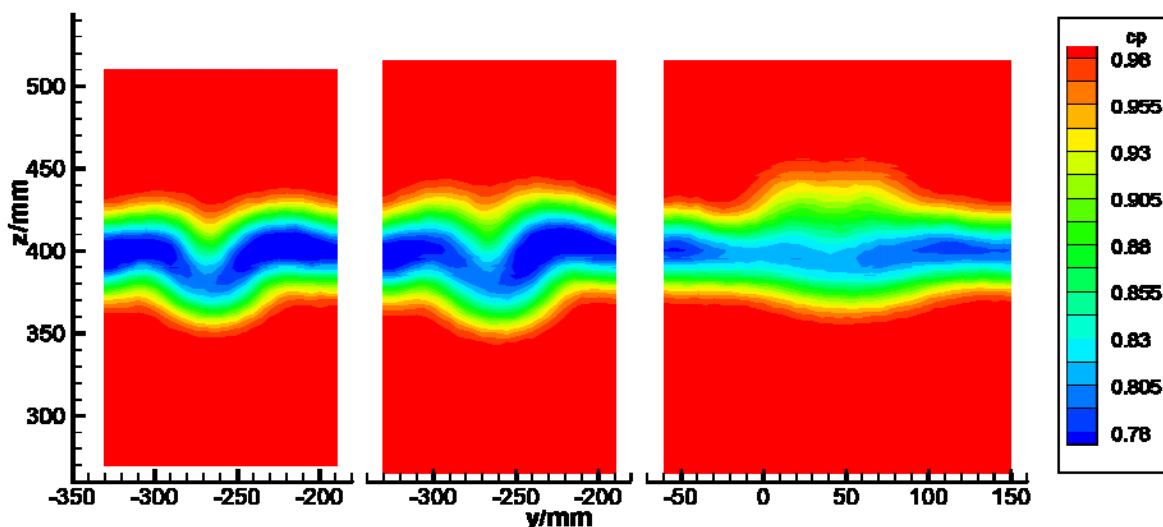
Fig. 12: Wake of fairings on the suction side: closed, open and cut at its maximum thickness
