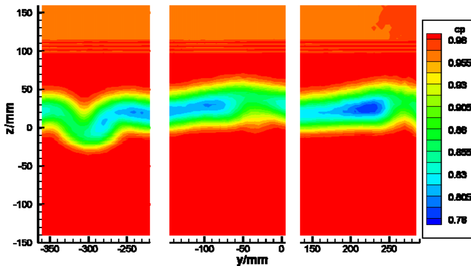
Fig. 10: Wake of covers (closed) on suction and pressure side
