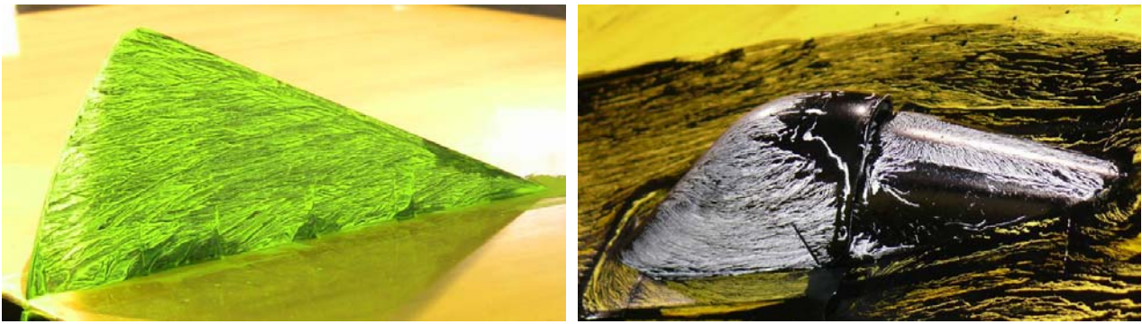
Fig. 8: Flow visualization on fence and aileron fairing
