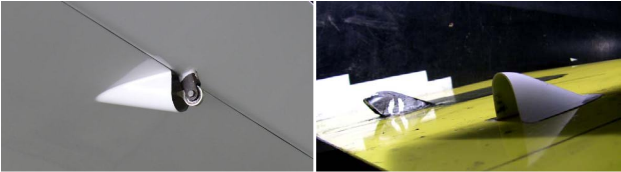
Fig. 11: Open fairings on Puchacz wing and w/t model
