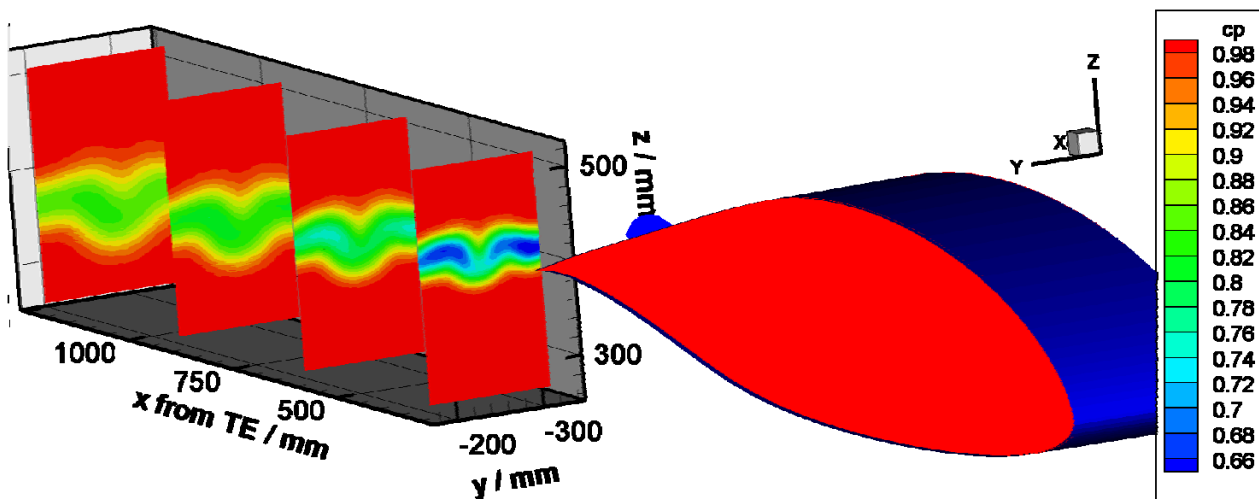
Fig. 13: Downstream development of the wake of a single aileron cover on the suction side of the wing
