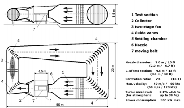
Fig. 2: Low speed wind tunnel of TU-DD
