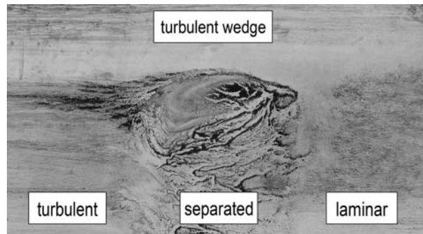
Fig. 5: Laminar separation on pressure side and turbulent wedge
