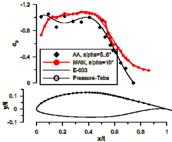
Fig. 3: Pressure distribution in wind tunnel and free flight
