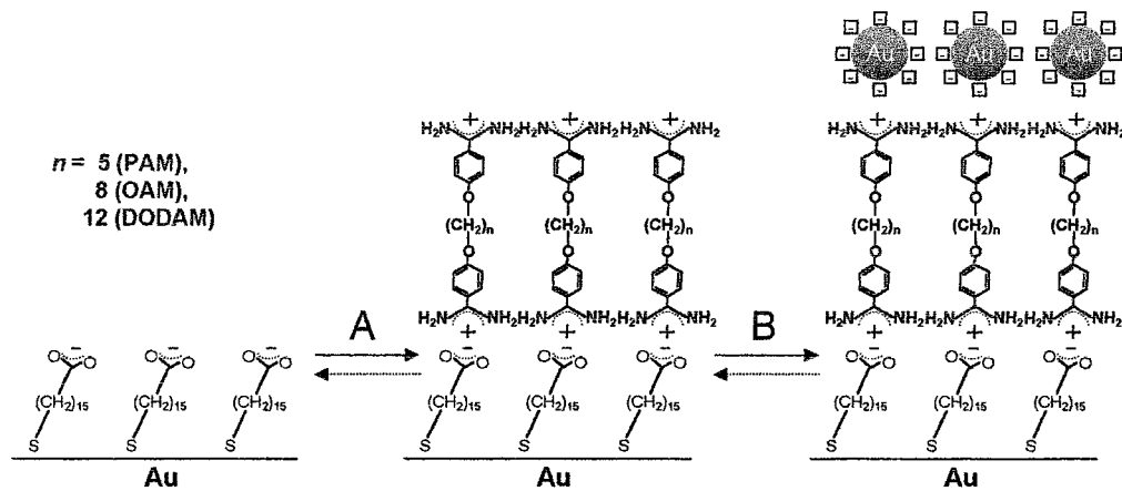
Figure 1. Schematic representation of the consecutive build-up of a SAM/nanoparticle composite by means of electrostatic interactions. Three different bis-benzamidines were used to serve as linking layers, n = 5 pentamidine (PAM), n = 8 octamidine (OAM), and n = 12 dodecamidine (DODAM).
