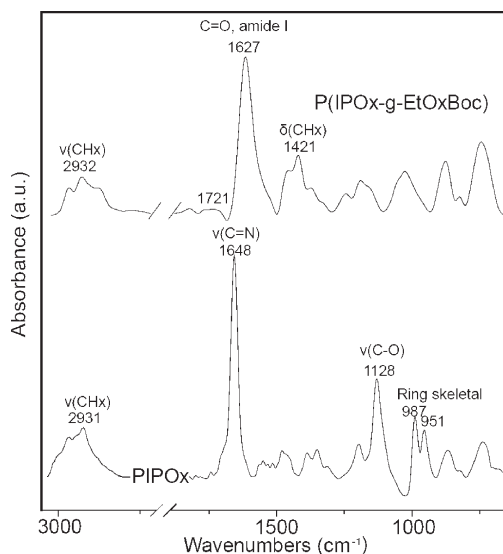
Figure 3. IR spectra of PIPOx and P(IPOx-g-EtOx) brushes on GC.
