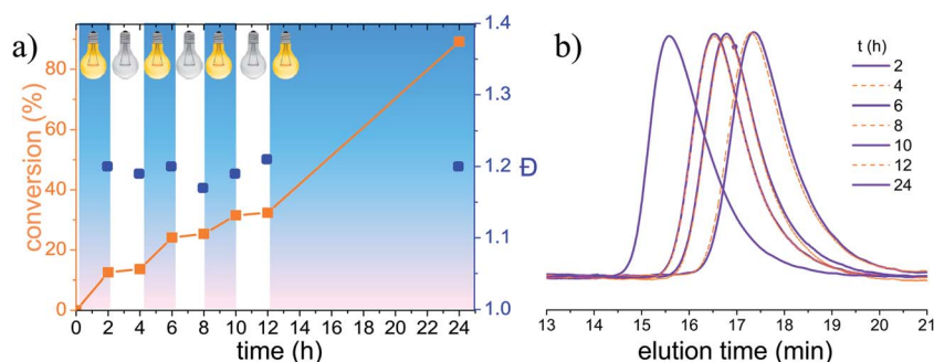
Fig. 4 Photoinduced ATRP performed by light–dark cycles of 2 h each. The stop-and-go characteristics of the polymerization is shown by (a) development of the monomer conversion as a function of the irradiation time over 24 h. Narrow dispersity is maintained throughout the experiment. (b) Development of M_n of the polymer product sampled at each time point as indicated in (a). Reactions were conducted with [\text{MMA}] : [\text{EBiB}] : [\text{CuBr}_2] : [\text{PMDETA}] = 100 : 1 : 0.1 : 0.3 at room temperature using irradiation from two fluorescent lamps at a distance of 10 cm to the reaction vial.
