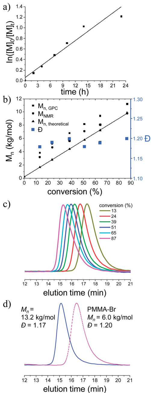
Fig. 2 Photoinduced ATRP of MMA. (a) First-order kinetic plot, (b) evolution of the polymer molar mass and dispersity, \bar{D} , with the monomer conversion and (c) respective GPC traces. Reactions were performed at a molar ratio of [MMA] : [EBiB] : [CuBr 2 ] : [PMDETA] = 100 : 1 : 0.1 : 0.3. (d) GPC traces for PMMA-Br used as a macroinitiator (pink) and resulting PMMA (blue) after 7 h irradiation of [MMA] : [PMMA-Br] : [CuBr 2 ] : [PMDETA] = 250 : 1 : 0.1 : 0.3. Reactions conditions for preparation of the PMMA-Br macroinitiator: time 5 h otherwise as for (c).
