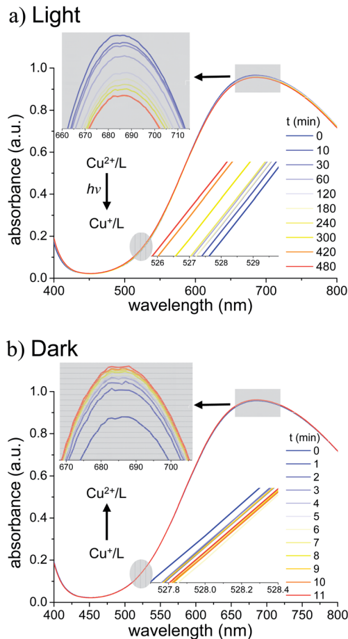
Fig. 3 In situ UV-vis spectroscopy of the Cu II /L system (EBiB ( 3.1 \times 10^{-2} M), CuBr 2 ( 3.1 \times 10^{-3} M) and PMDETA ( 9.3 \times 10^{-3} M) in DMF-methanol (v/v, 2/1)). (a) Spectra recorded during irradiation with visible light (400–750 nm) in a quartz cell at room temperature; (b) UV-vis spectral changes in the dark.
