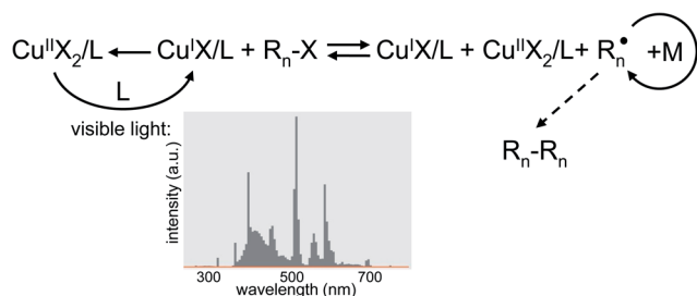
Fig. 1 Reaction mechanism for the photoinduced ATRP. Even light in the visible range as emitted by a standard fluorescent lamp (type L58W/880 "SKYWHITE" from Osram®, Germany, emission spectrum as provided by the manufacturer) is able to close the Cu II /Cu I redox cycle. Such lamps are a common light source and also used to illuminate laboratory hoods.
