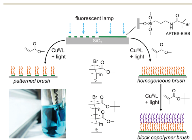
Fig. 5 Photoinduced surface-initiated ATRP (PSI-ATRP) of MMA on a SAM of APTES-BIBB on silicon dioxide. The initiator-SAM was prepared as reported by Cui et al. 22 Patterned polymer brushes were prepared from photopatterned initiator-SAMs and block copolymer brushes by consecutive PSI-ATRP reactions. The photograph in the lower left corner shows the experimental setup.
