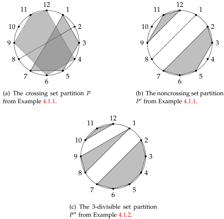
FIGURE 39. Cycle diagrams of set partitions.
