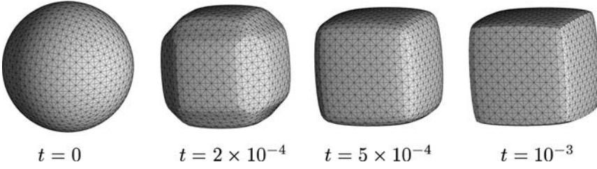
Fig. 2. Evolution of a sphere with volume V=1.0 towards its steady state with anisotropy (13). No space/time adaptivity: 1538 grid points and time step \tau=10^{-5} . The surface is shown at times t=0 , t=2 \times 10^{-4} , t=5 \times 10^{-4} , t=10^{-3} . Note that the rounded corners of the Wulff shape in Fig. 1 are not properly resolved in the steady state ( t=10^{-3} ) since the spatial discretization is not fine enough.
