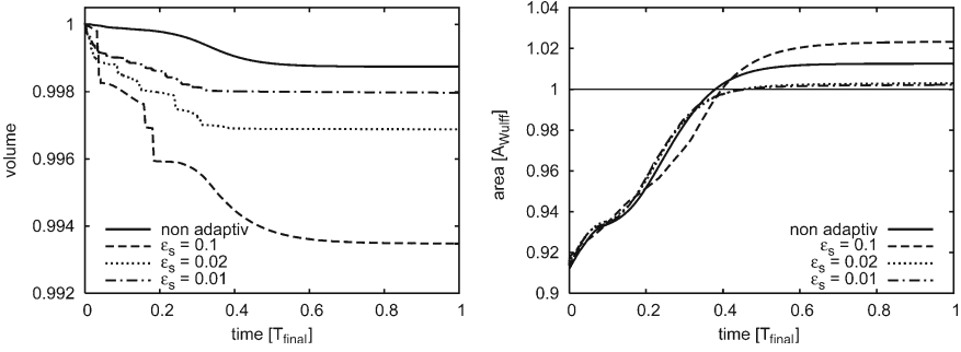
Fig. 5. Evolution of a sphere with volume V = 1.0 towards its steady state with anisotropy (13). (left) Volume versus relative time t/T_{\text{final}} ( T_{\text{final}} = 2 \times 10^{-3} ); the volume is conserved within less then 1% in all simulations. (right) Relative area A/A_{\text{Wulff}} versus relative time, where A_{\text{Wulff}} is the area of the Wulff shape with volume V(T_{\text{final}}) ; (for V = 1 , A_{\text{Wulff}} \approx 5.3097 ). The area of the steady state approaches A_{\text{Wulff}} for small \varepsilon_s very accurately.
