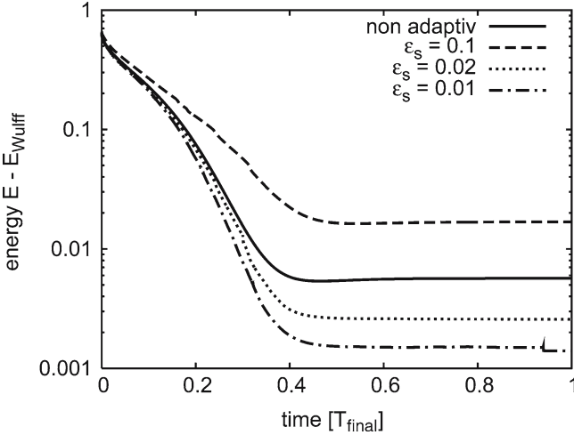
Fig. 6. Evolution of a sphere with volume V = 1.0 towards its steady state with anisotropy (13). Surface energy E - E_{\text{Wulff}} versus relative time, where E_{\text{Wulff}} is the surface energy of the Wulff shape with volume V(T_{\text{final}}) ; (for V = 1 , E_{\text{Wulff}} \approx 6.8922 ). The surface energy decays exponentially and the energy of the steady state approaches E_{\text{Wulff}} with decreasing tolerance \varepsilon_s .
