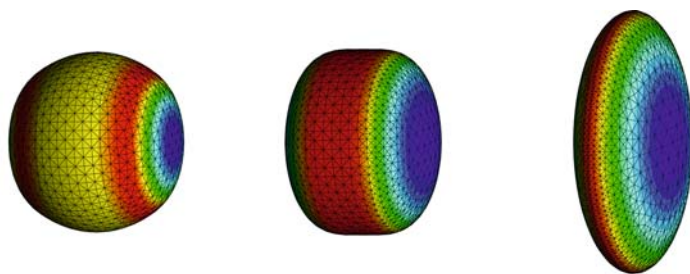
Fig. 7. Evolution of a sphere towards its steady state with anisotropy (14) and element tolerance \varepsilon_s = 0.02 . The number of grid points is given between parentheses. The color-coding indicates the normal velocity (rescaled), ranging from red (maximal outwards) over yellow to blue (maximal inwards).
