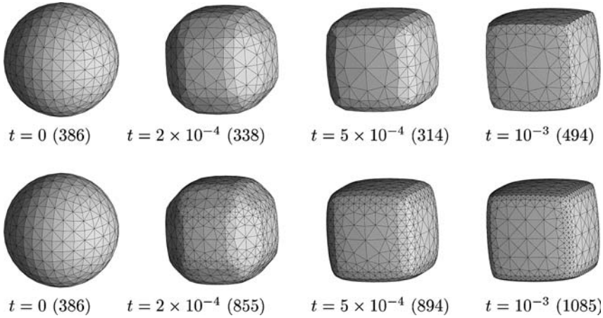
Fig. 3. Evolution of a sphere with volume V = 1.0 towards its steady state with anisotropy (13). Refinement in regions of high curvature and coarsening in nearly flat regions (the number of grid points is given between parentheses). (Top row) element tolerance \varepsilon_s = 0.1 , (bottom row) \varepsilon_s = 0.05 .
