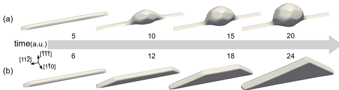
Figure 10. Selective-area growth of GaAs crystal in a pure thermodynamic regime (a) and in a kinetic regime (b) with \tau_{110} = 100 and \tau_{111} = 10 . The surface energy is anisotropic with \gamma_{111B} = 0.89 , \gamma_{111A} = 0.99 , \gamma_{110} = 0.90 , \gamma_{100} = 0.90 . Corner regularization is used with \beta = 0.001 . Material is deposited with a flux distribution at a 45^\circ angle.
