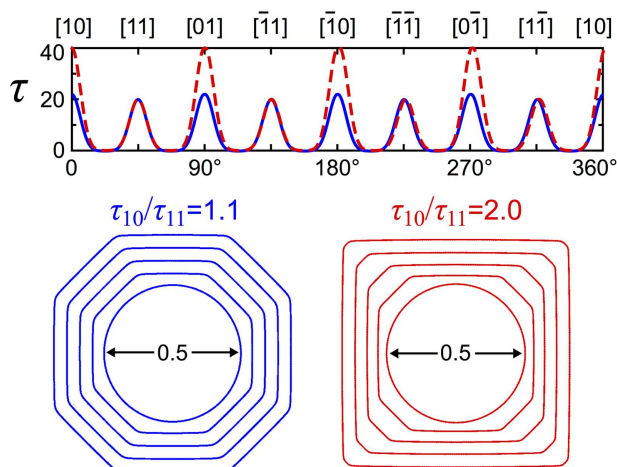
Figure 4. Comparison of the shape evolution from circular to faceted shape for different \tau_{10}/\tau_{11} ratios, by using the anisotropy functions shown in the top panel.
