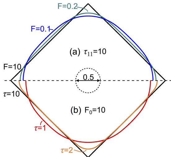
Figure 6. Comparison of the out-of-equilibrium conditions needed for the kinetic faceting. a) Profiles obtained by changing the deposition flux, for a fixed \tau_{11} . b) Profiles obtained by changing \tau_{11} , for the same F_0 = 10 . All the profiles have the same volume, and the initial stage is a circle. M_0 = 0.1 .
