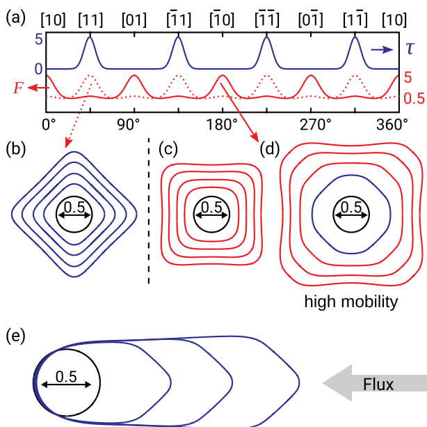
Figure 8. Combination of anisotropic incorporation time and material supply. a) Plot of the F(\hat{n}) and \tau(\hat{n}) anisotropy functions used. b) Both anisotropies lead to the \{11\} square ( M_0 = 0.001 ). c) The flux anisotropy is rotated by 45^\circ (dotted line in panel (a)) and imposes \{10\} faceting ( M_0 = 0.001 ). d) The mobility is increased ( M_0 = 0.007 ), while keeping the opposite anisotropies for flux and kinetics as in (c). e) The flux F_0 = 0.5 is directed on one side of the crystal, following the arrow.
