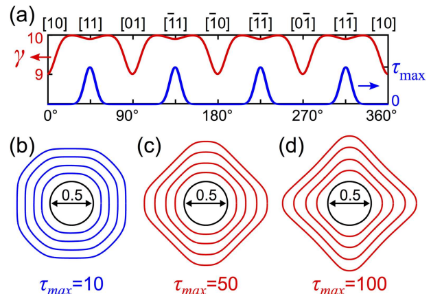
Figure 7. Competing role of incorporation time and surface energy anisotropy. For larger \tau (center and right) the kinetic faceting dominates over the thermodynamic one resembling the ECS (left). Corner regularization is used with \beta = 0.05 , while the anisotropy functions for \tau(\hat{n}) and \gamma(\hat{n}) are plotted in the top panel.
