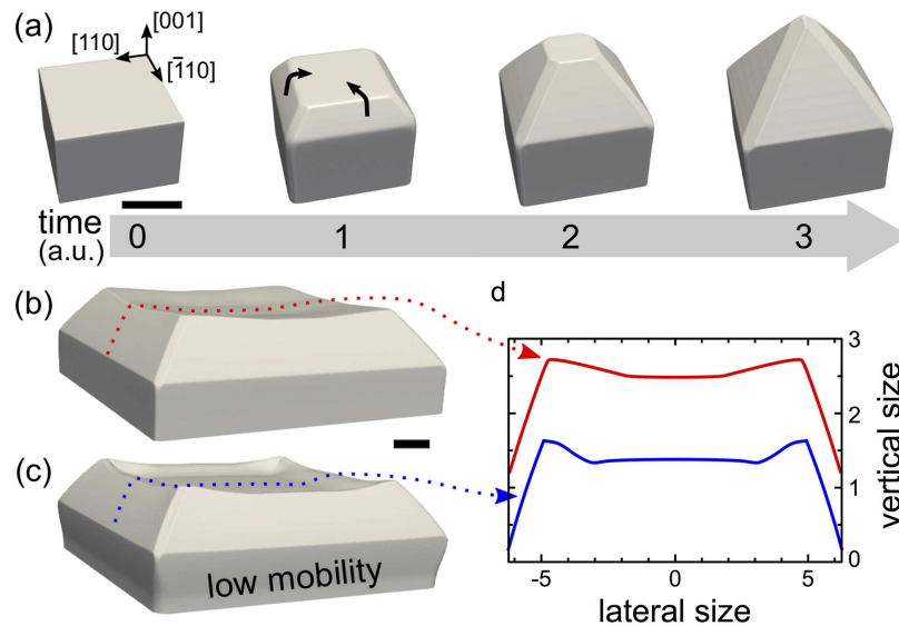
Figure 9. a) Time evolution of a pillar top with competing incorporation times for the top (001) and the lateral {111} and \{1\bar{1}0\} . b) and c) Comparison of the growth on a four-times larger base for two different mobility coefficients ((c) 10 times smaller). d) Comparison of the central (110) cross-sectional profiles, shifted arbitrarily in the vertical direction. The flux F_0 = 0.5 is vertical, \tau_{110} = \tau_{111} = 10 , \tau_{001} = 1 . The scale bar is 1.5 length units.
