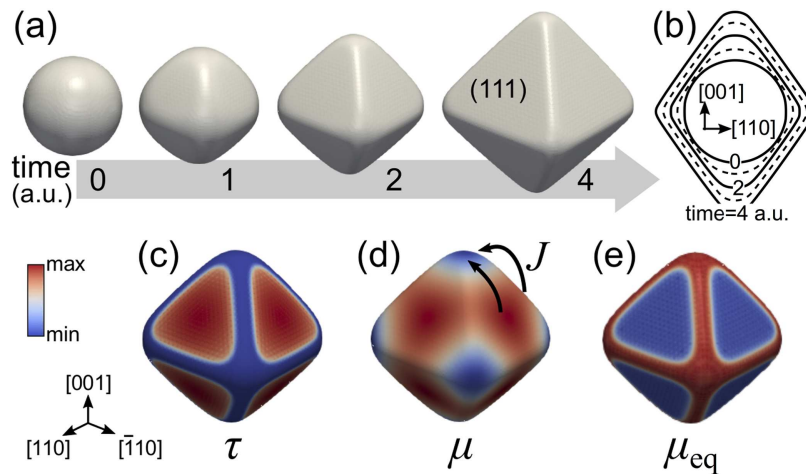
Figure 2. a) Growth simulation of a {111} faceted shape with the kinetic incorporation term. b) Time evolution of cross-section profiles. Color map for (c) the incorporation time \tau , (d) the chemical potential \mu and (e) the equilibrium chemical potential \mu_{eq} , corresponding to the surface curvature. \tau_{111} = 20 and M_0 = 0.1 .
