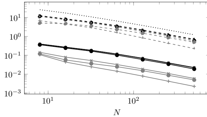
FIG. 4.2. Convergence behaviour in the energy norm (solid line) and the balanced norm (dashed line) for \varepsilon_1 = 10^{-8} ( \bullet ), 10^{-9} ( + ), and 10^{-10} ( \times ) and \varepsilon_2 = 10^{-3} (black) and 10^{-4} (gray).
