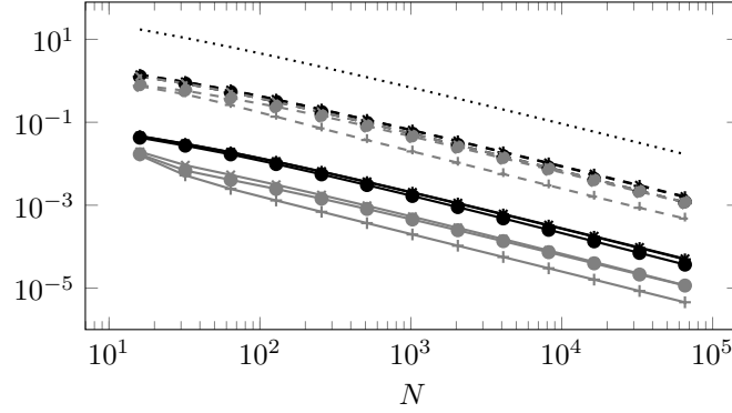
FIG. 4.1. Convergence behaviour in the energy norm (solid line) and the balanced norm (dashed line) for \varepsilon_1 = 10^{-8} ( \bullet ), 10^{-9} ( + ), and 10^{-10} ( \times ) and for \varepsilon_2 = 10^{-3} (black) and 10^{-4} (gray).
