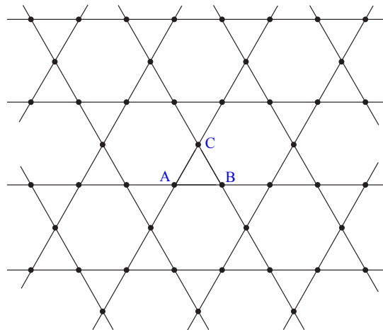
Figure 1: The kagome lattice.
