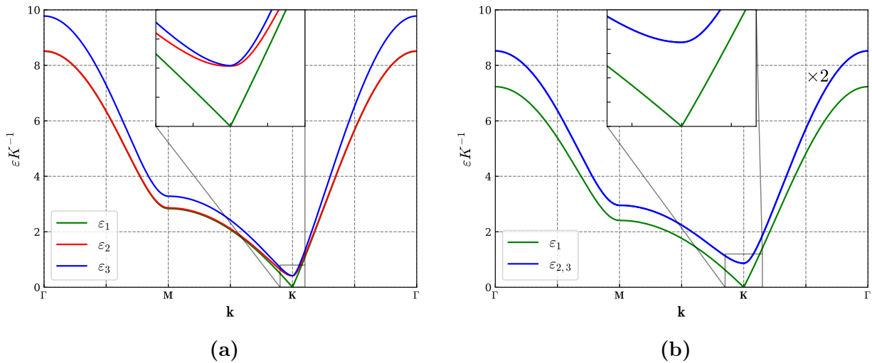
Figure 5.2: Representative spectra for (a) the U(1) SSB phase at (J_{xy}, J_z) = (0.6, 0.2) and (b) the \mathbb{Z}_2 SSB phase at (J_{xy}, J_z) = (0.2, 0.6) . Spectrum (a), which is adiabatically connected to the ordered phase of the Kitaev-XY spin-orbital model and thus shares the same qualitative features as the dispersion in Fig. 4.2b. Spectrum (b) features two degenerate gapped with one remaining Dirac cone, a defining feature of the \mathbb{Z}_2 symmetry-broken phase.
