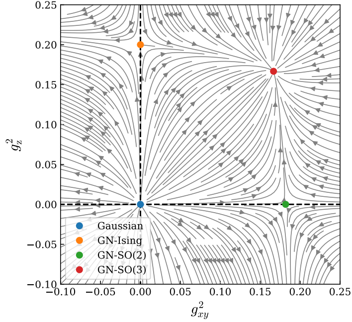
Figure 5.7: RG flow of the anisotropic Gross-Neveu-SO(3) model in the bicritical manifold. The IR stable fixed point is GN-(SO(2)+I)*, featuring an emergent SO(3) symmetry. The quantum critical points GN-SO(2)* and GN-Ising* are retained in the XY and Ising limit, respectively.
