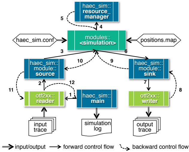
Figure 3: Software control flow in HAEC-SIM.
